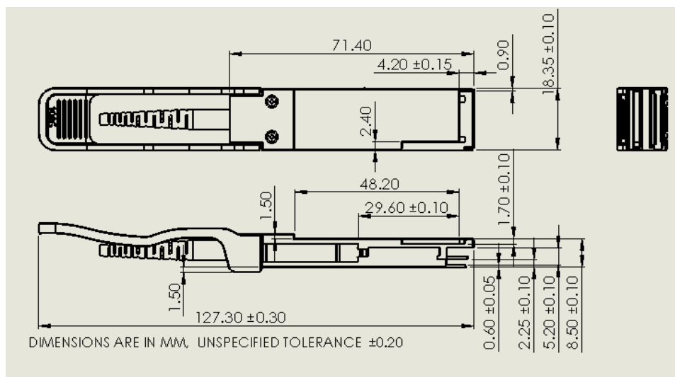
Figure 6. Mechanical Outline
