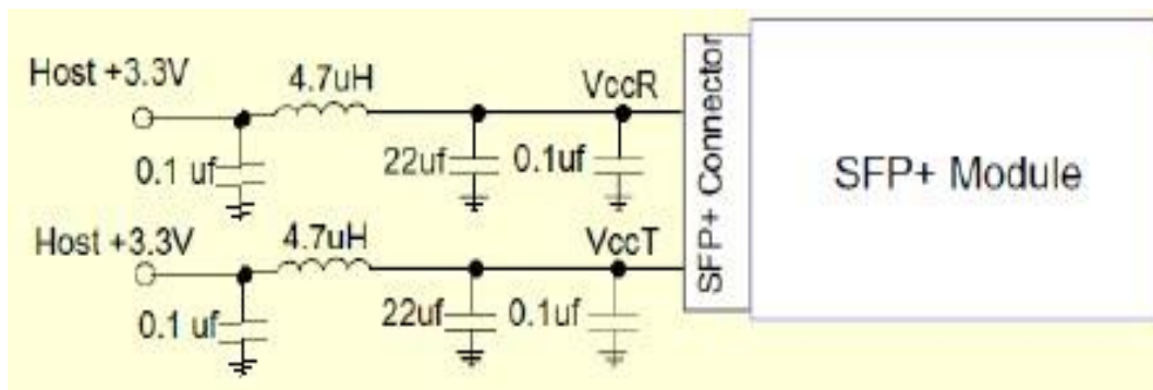
Recommended Host Board Power Supply Circ
