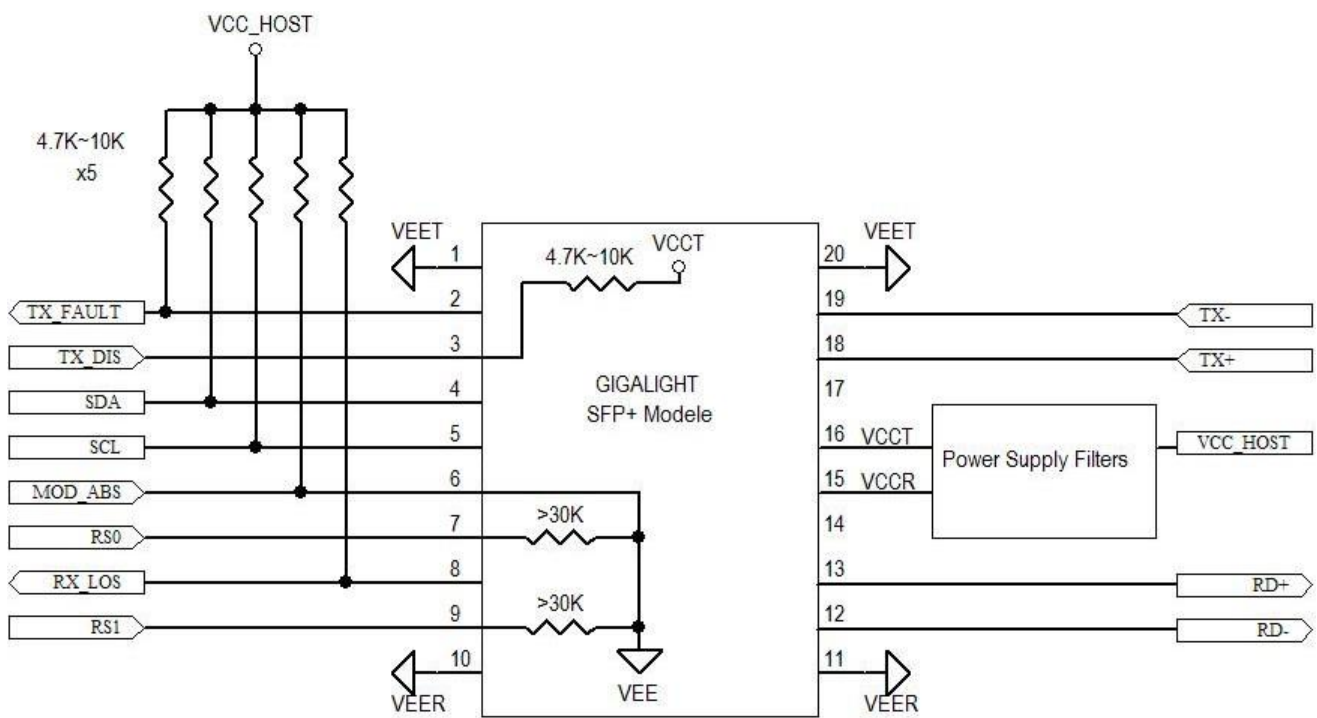
Figure4. Host-Module Interface
