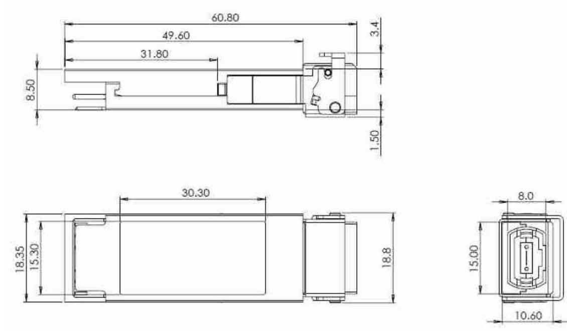
Figure6. Mechanical Specifications
