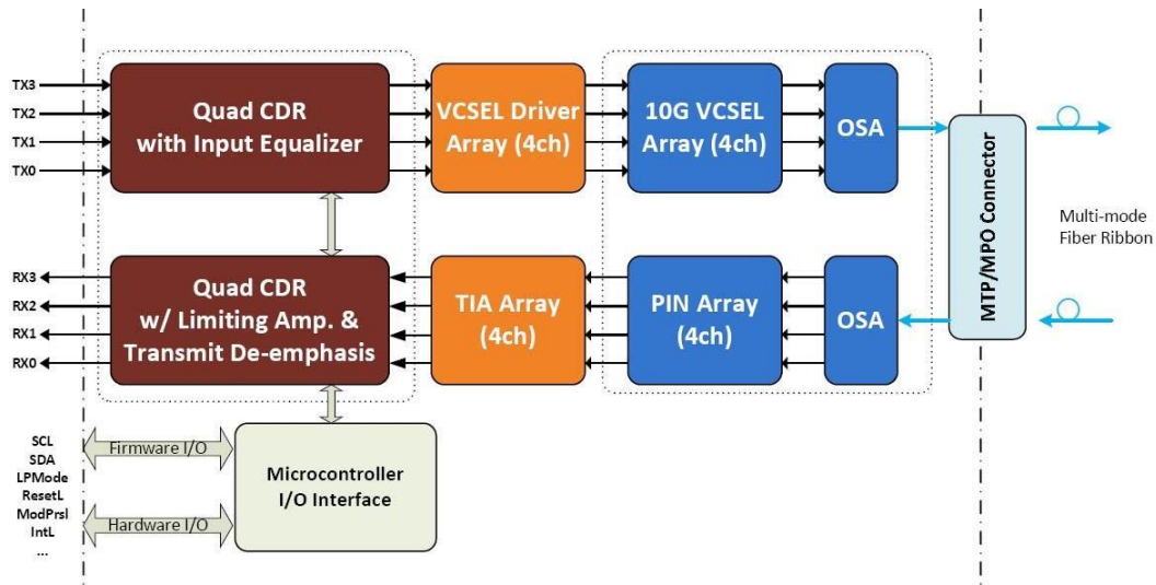
Figure1: Block Diagram
