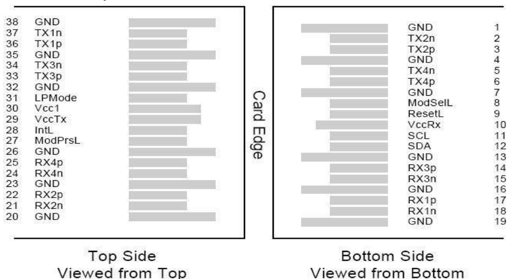
Figure 2. MSA Compliant Connector
