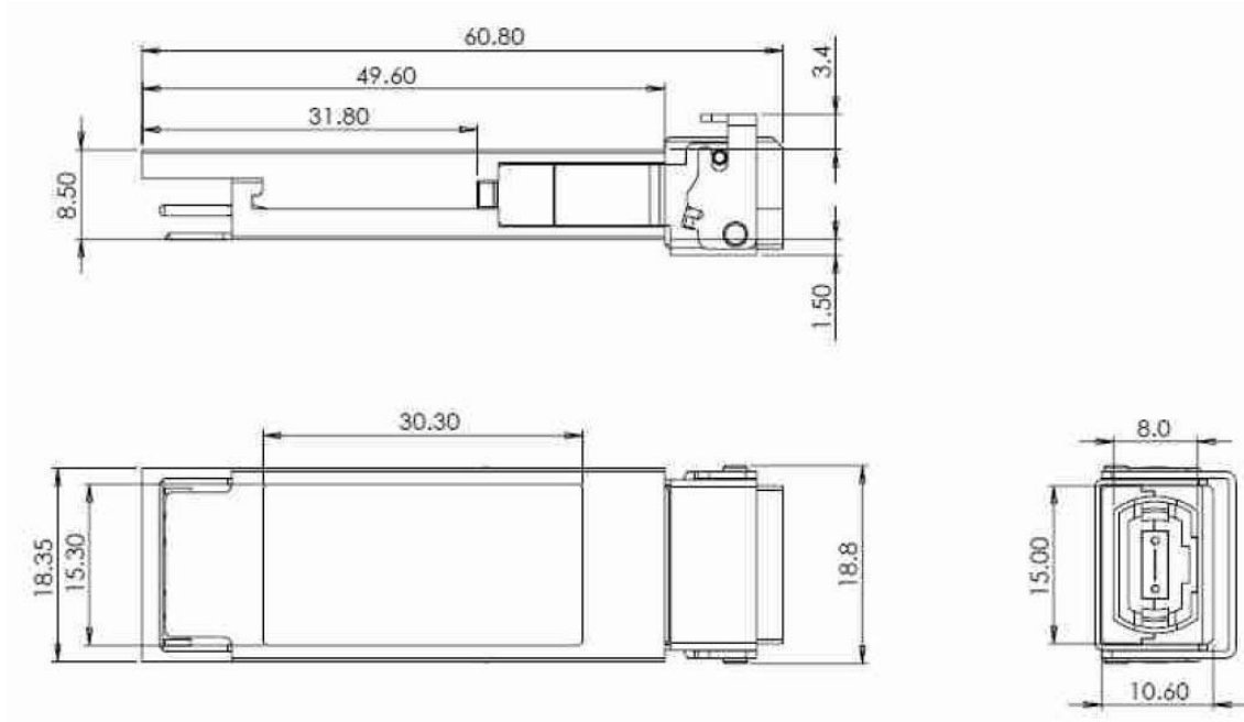
Figure6. Mechanical Specifications
