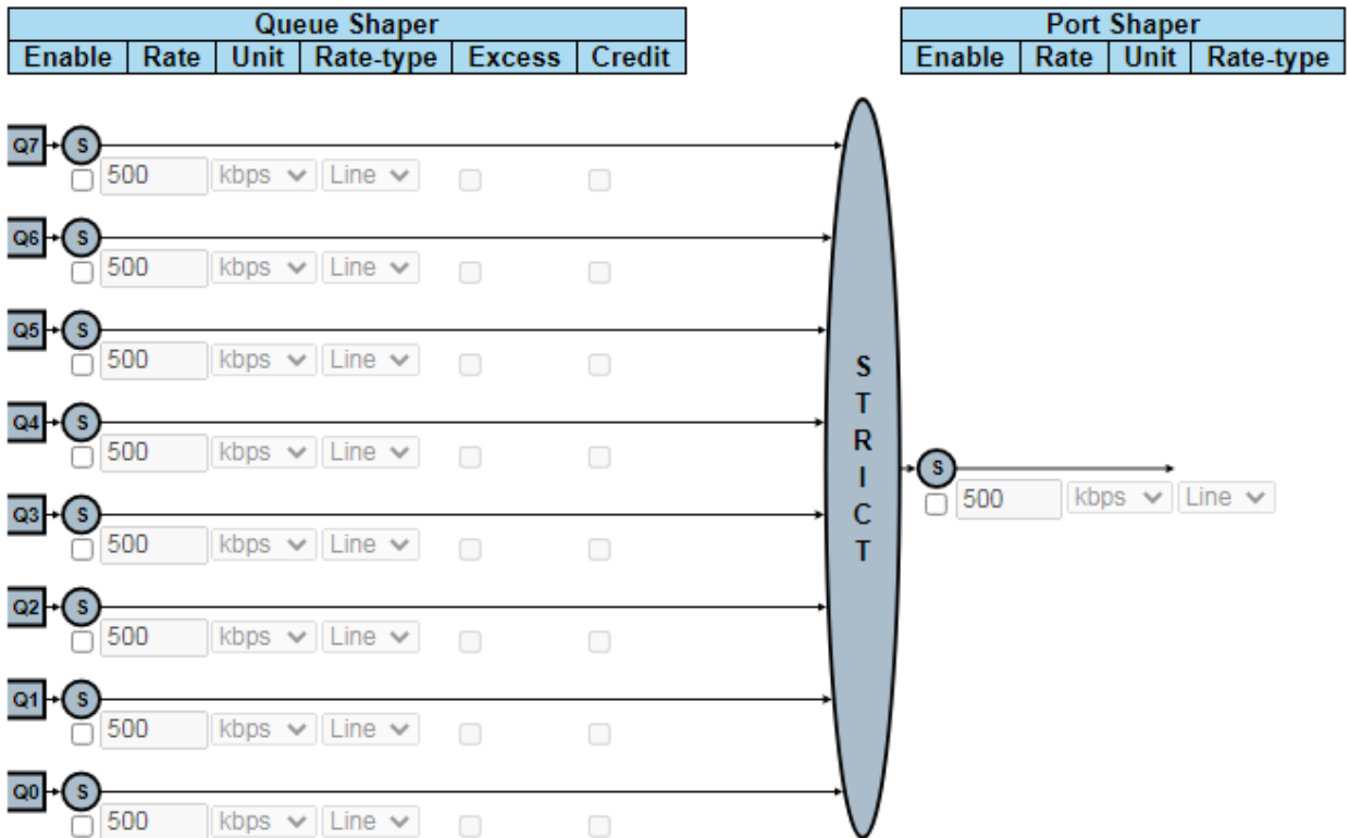
Рис. 3.103 – Port Scheduler
