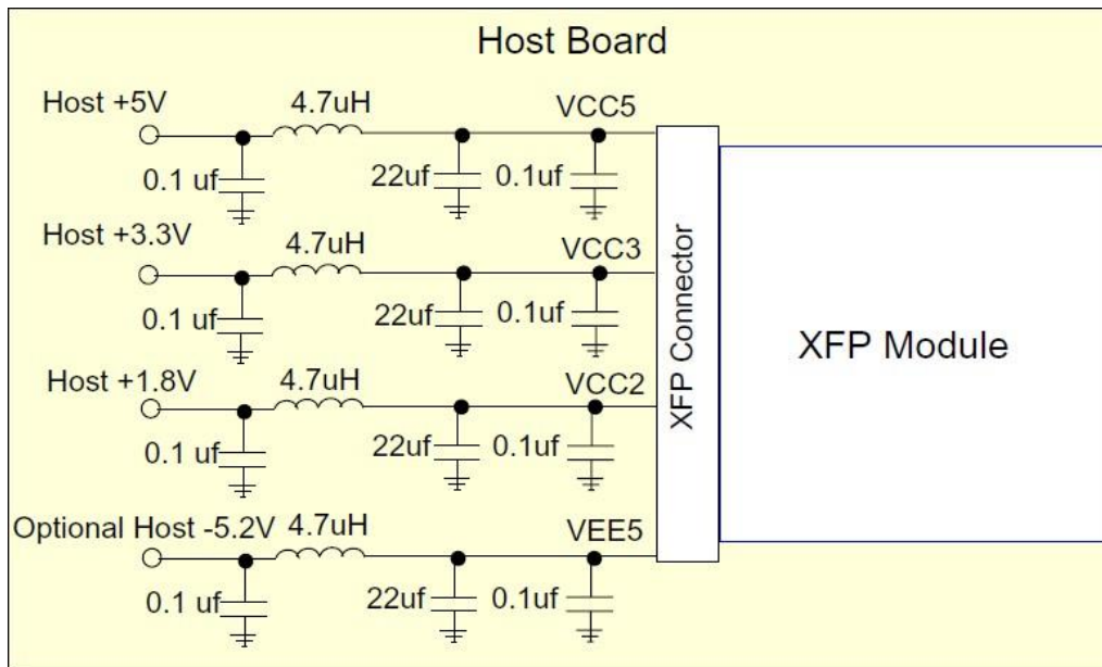
Recommended Host Board Power Supply Circuit
