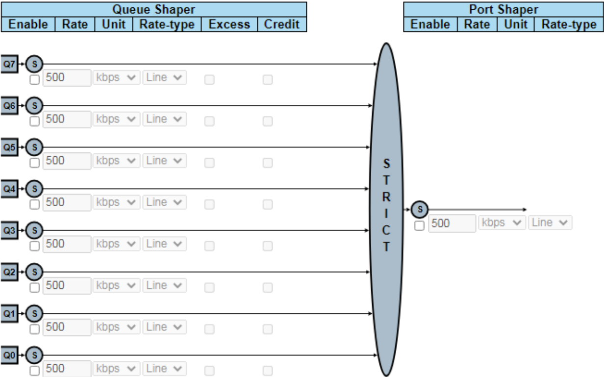
Рис. 4.2.40.3 – Port Scheduler
